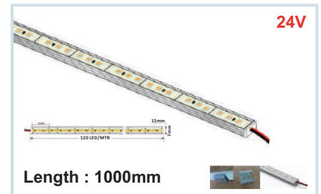
HLO-7020 (9.6W/Mtr) Size : 1000x15x7mm LED RIGID STRIP LIGHT
