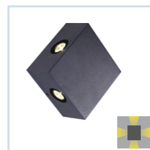
HLO-5354 (4x1W) Size : 100x100x52mm
