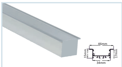
HLL-1062 : CONCEALED BODY - FULL SET STANDARD LENGTH : 2MTR SIZE : 46xD17mm / CUT-OUT : 34xD15mm
