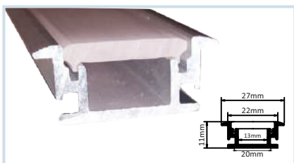
HLL-1072 : GROUND FLOORING CONCELD STANDARD LENGTH : 3MTR SIZE : 27xD11mm / CUT-OUT : 20xD8mm
