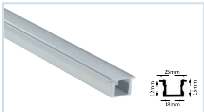
HLL-1056 : CONCEALED BODY - FULL SET STANDARD LENGTH : 2MTR SIZE : 25xD15mm / CUT-OUT : 18xD12mm
