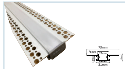
HLL-1126 : CONCEALED BODY - FULL SET STANDARD LENGTH : 2MTR SIZE : 73xD16mm / CUT-OUT : 31xD14mm
