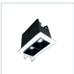
HLR-2931 (3W) Size : 52x32mmx40mm Cut-Out : 48x27mm Body Colour Available : White / Black
