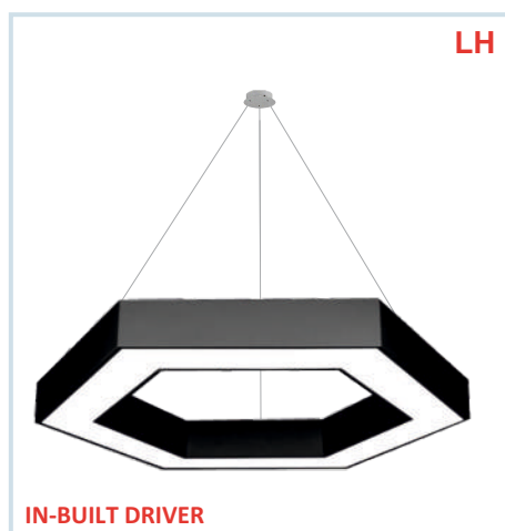
HLL-1866 (20W) Size : ⬡450xW36xH65mm
