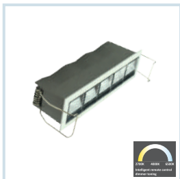
HLR-2930 (15W) Size : 165x50mmx45mm Cut-Out : 155x35mm
