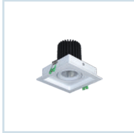
HLR-2608 (1x15W) Size : 110x110x98mm Cut-Out : 95x95mm
