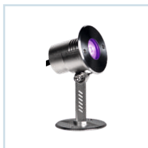
HLO-6502 (3W) - RGB Size : Ø68.5x73x132mm
