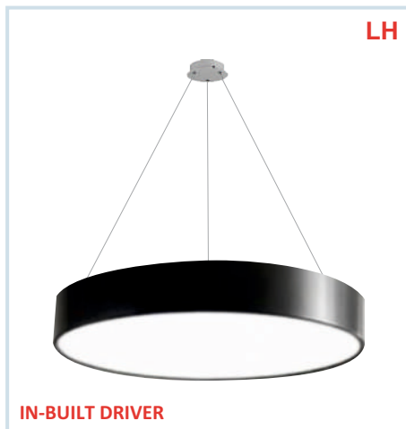
HLL-1862 (20W) Size : Ø450xH75mm
