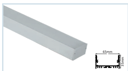
HLL-1015: SURFACE BODY - FULL SET STANDARD LENGTH : 2MTR SIZE : 65x35mm
